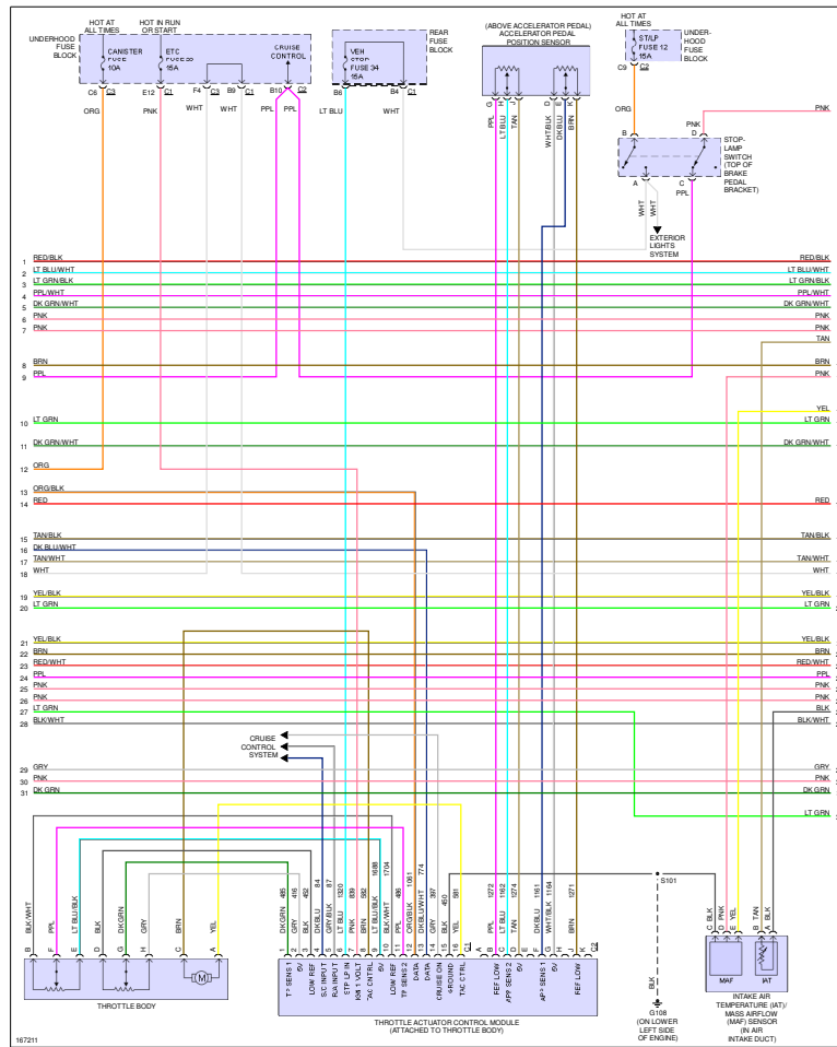
Fig 4: 5.3L VIN P, Engine Performance Circuit (4 of 5)
