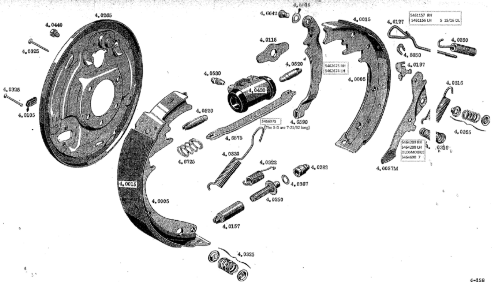
HYDRAULIC REAR BRAKE 1000, K1000-F SERIES (SPICER 44, 60-35 AXLES)
