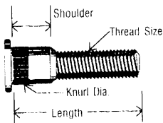
SERRATED BOLTS
