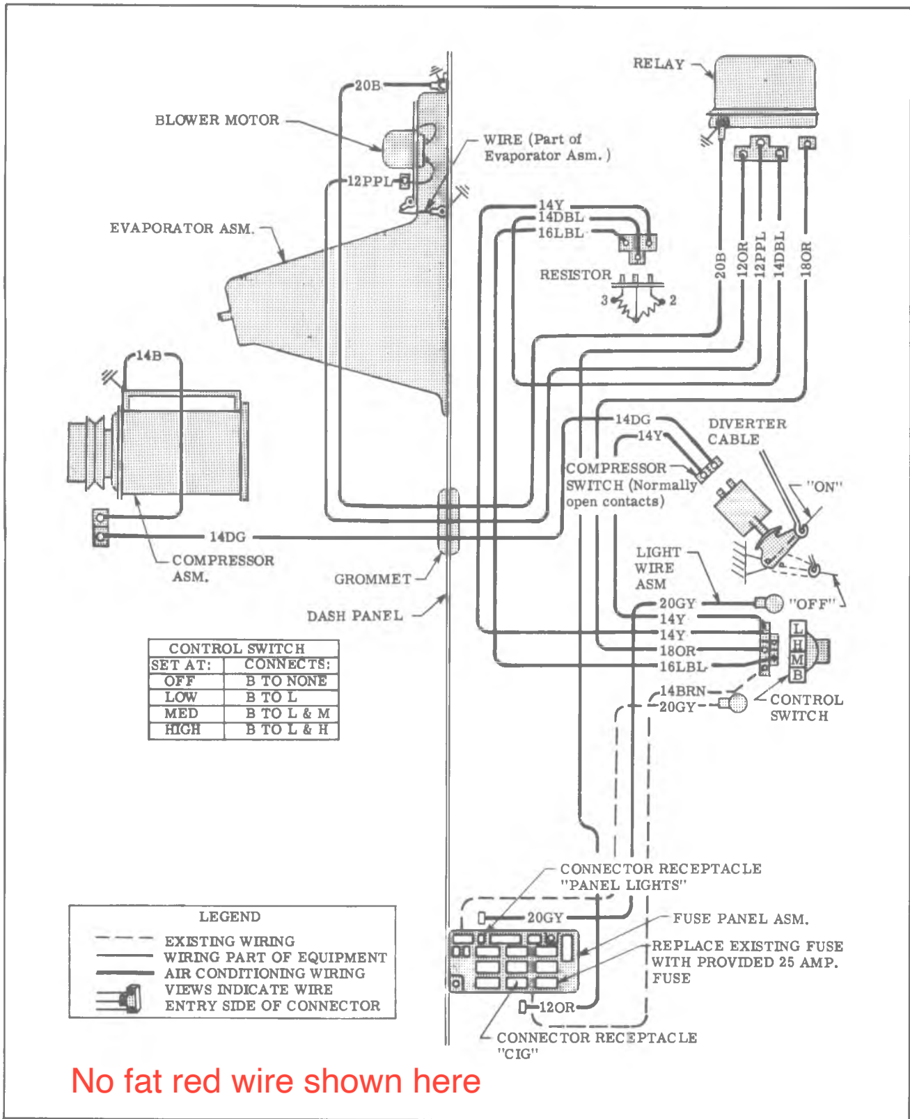
Fig. 64—Four-Season System Wiring Diagram
