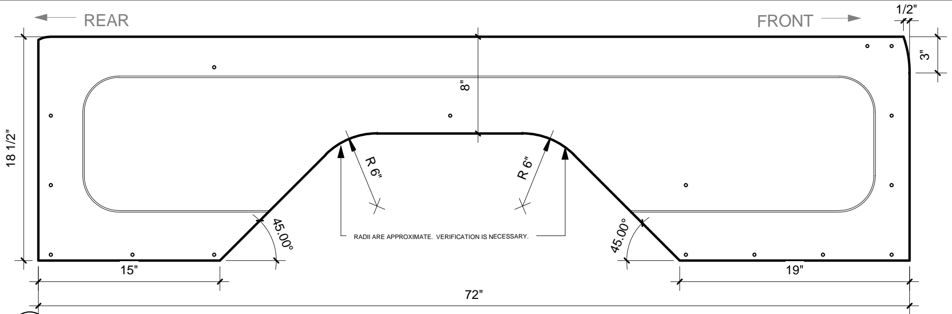
1 DRIVER SIDE PANEL 1 1/2" = 1'-0"
