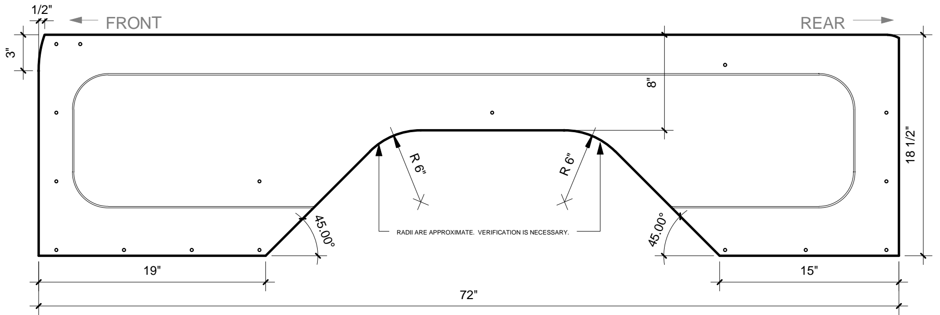
2 PASSENGER SIDE PANEL 1 1/2" = 1'-0"
