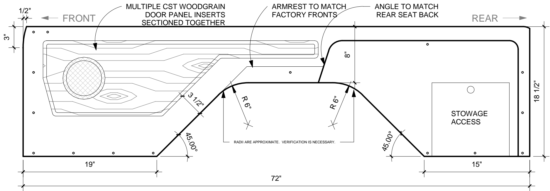
1 DRIVER SIDE PANEL - OPTION 1 1 1/2" = 1'-0"
