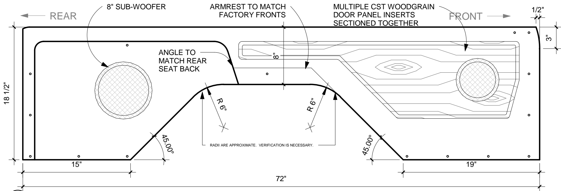
1 DRIVER SIDE PANEL - OPTION 1 1 1/2" = 1'-0"
