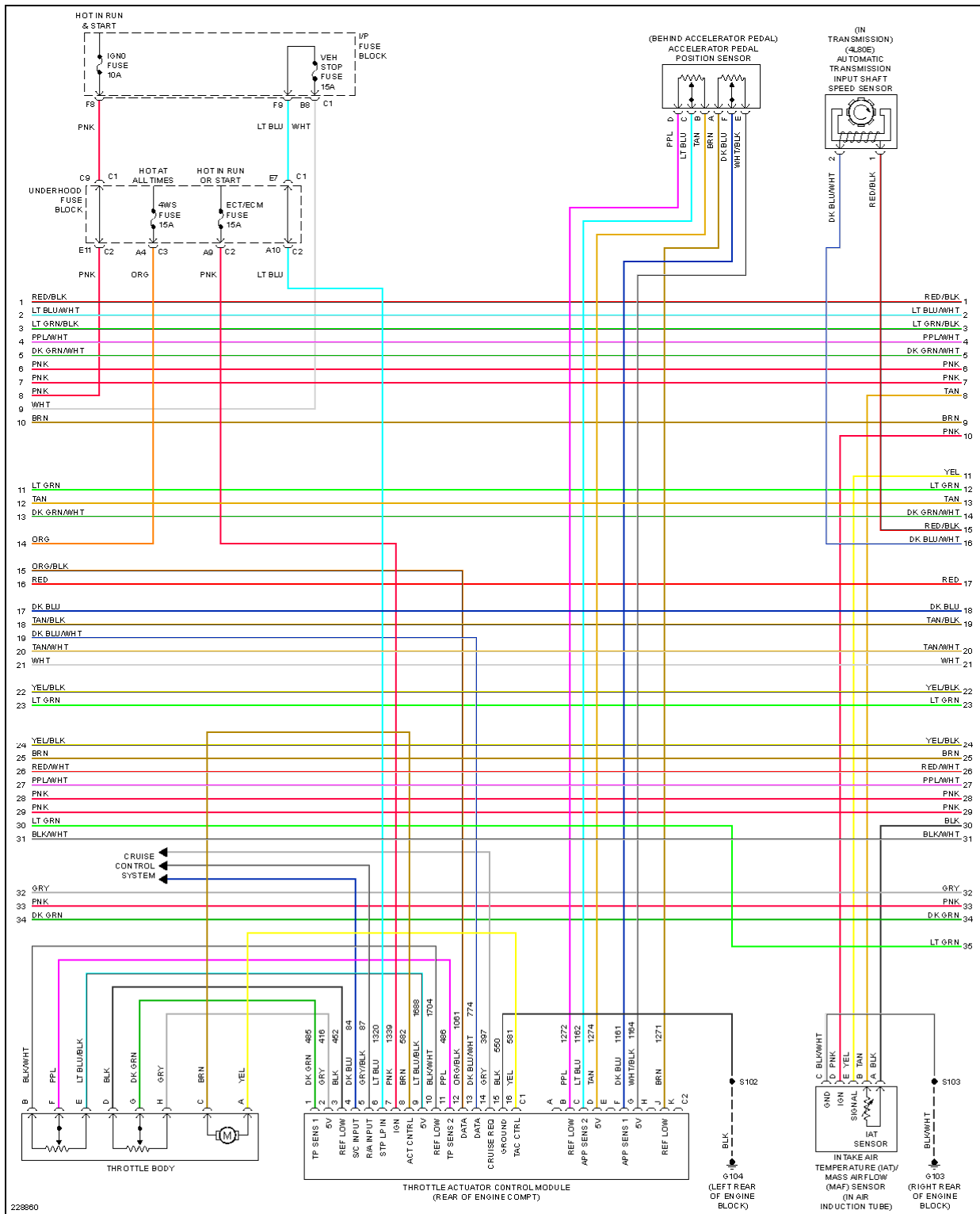
Fig. 45: 6.0L VIN U, Engine Performance Circuit (4 of 5)
